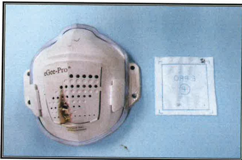
Photograph 2 eGee-Pro Mask with antibacterial refill filter after flammability test
